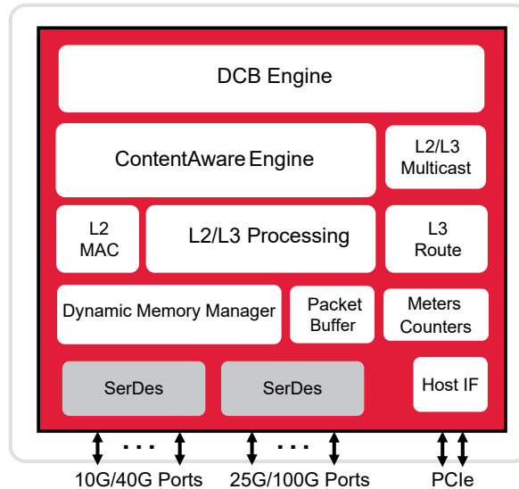
Figure 1: BCM56760 Block Diagram
