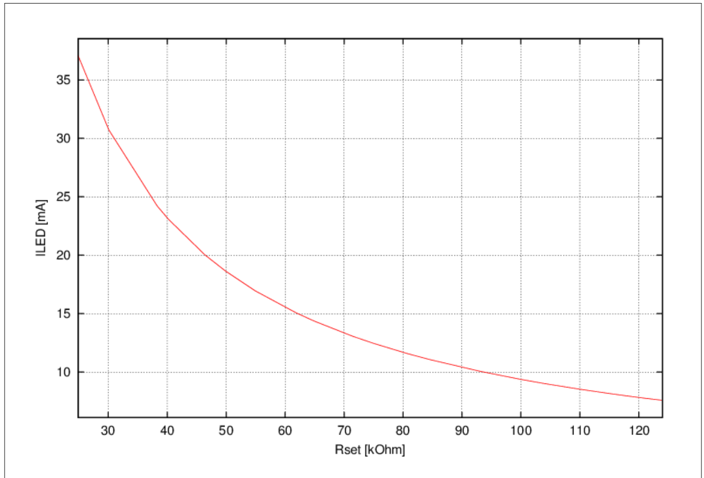
Figure 3 Relation between I_{LED} and R_{set}
