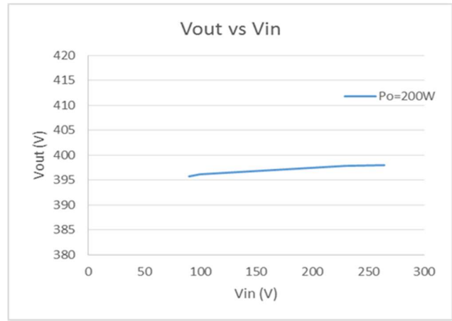
Figure 9. Line Regulation ( V_{OUT} vs V_{IN} )
