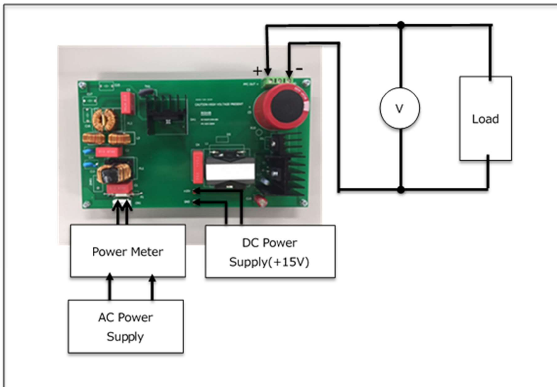
Figure 1. Connection Circuit
