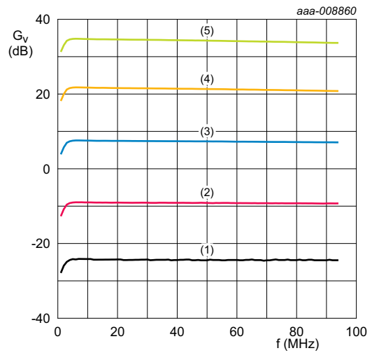
aaa-008860 V_{CC} = 5 \text{ V} ; current setting = 3; T_{amb} = 25 \text{ }^\circ\text{C} ; P_i = 30 \text{ dBmV} . (1) gain setting = 5 (2) gain setting = 20 (3) gain setting = 36 (4) gain setting = 50 (5) gain setting = 63
