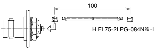
BNC(75)J-H.FLJ-BPA(40)
