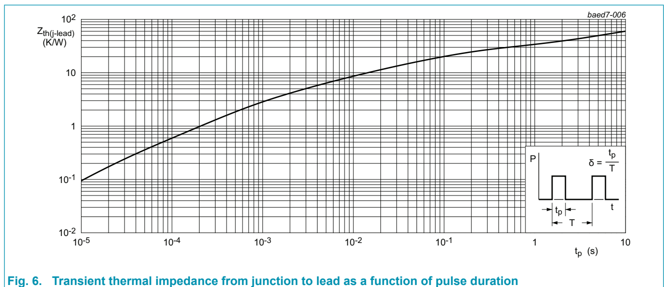
Fig. 6. Transient thermal impedance from junction to lead as a function of pulse duration
