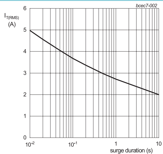
Fig. 2. RMS on-state current as a function of surge duration; maximum values f = 50\text{ Hz} ; T_{lead} = 57\text{ °C}
