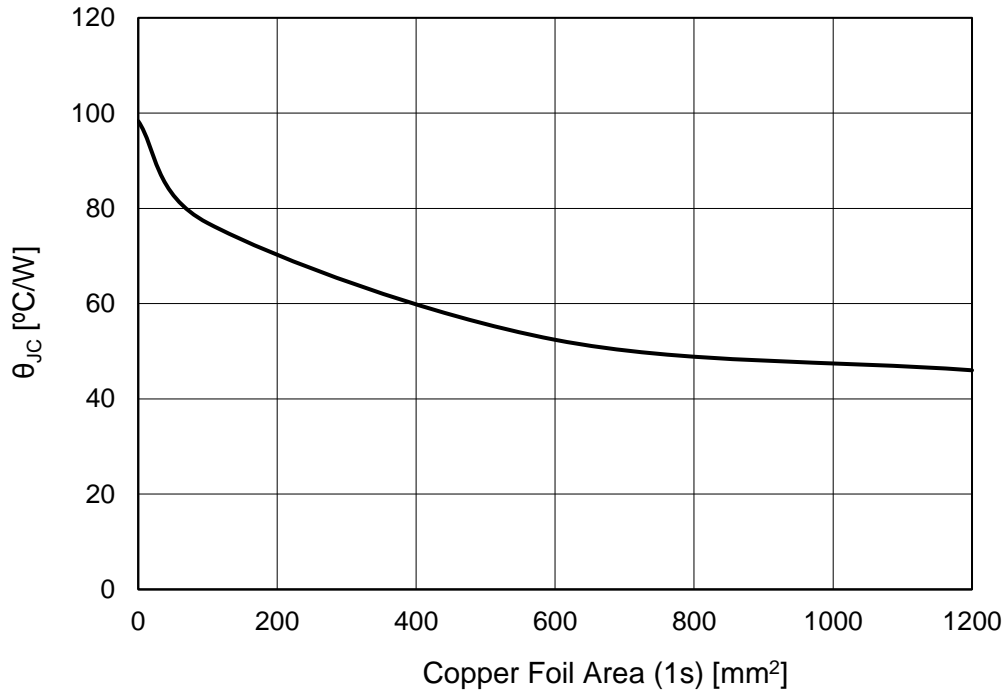
Figure 10. Thermal Resistance
