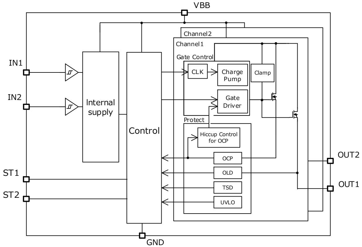
Figure 3. Block Diagram
