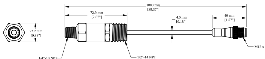
BWA-PRESSURE-SENSOR-50 and -150 gauge models
