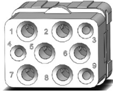
Insert Name 09 Insert Code D 3 x size 20 contacts 6 x size 15 or 16 contacts
