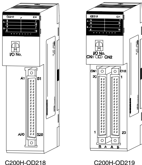
C200H-OD218
