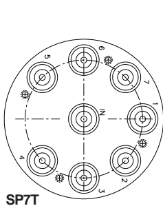
SP7T
