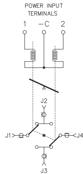
SCHMATIC
