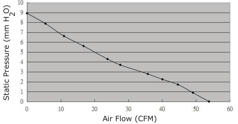
CFM-8020BF-255-444
