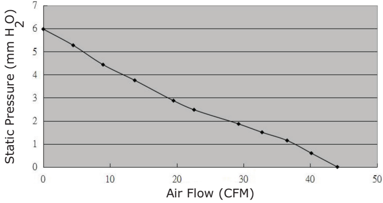
CFM-8020BF-245-401
