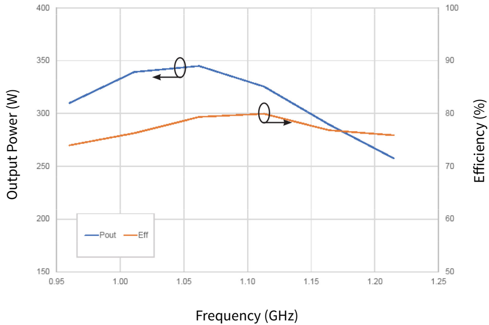
Figure 6. Pulsed Output Power and Drain Efficiency vs. Frequency of the CGHV40180F-AMP3 V_{DD} = 50\text{ V} , I_{DQ} = 1.0\text{ A} , P_{IN} = 38\text{ dBm} , 128\ \mu\text{s} , 10% pulse
