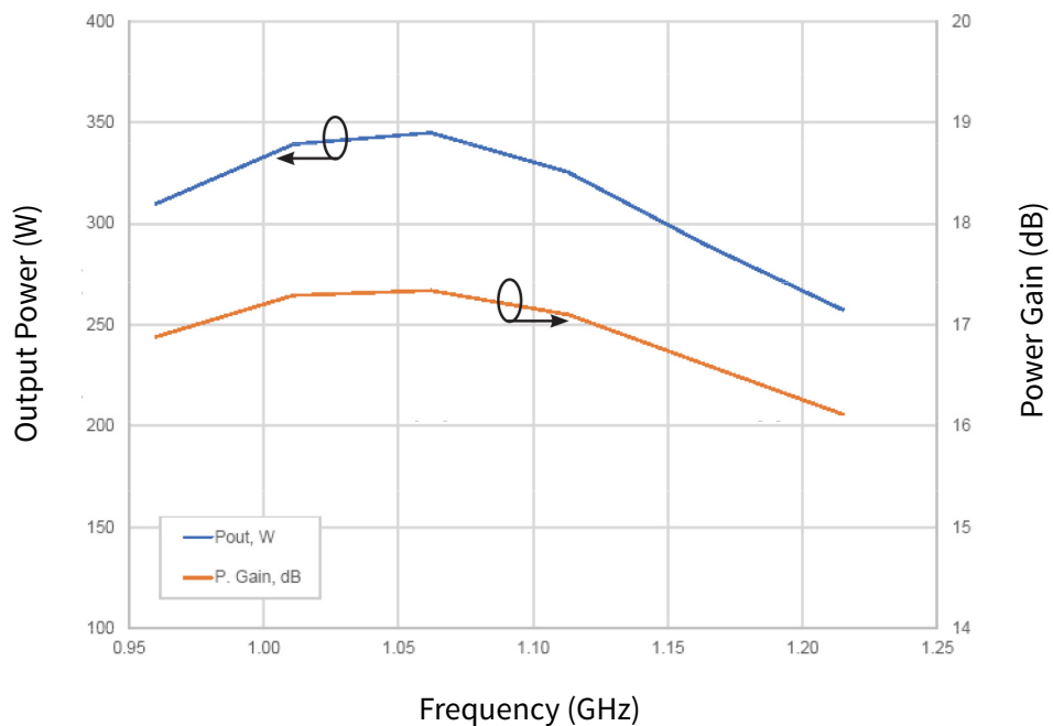
Figure 7. Output Power and Power Gain vs. Frequency of the CGHV40180F-AMP3 V_{DD} = 50\text{ V} , I_{DQ} = 1.0\text{ A} , P_{IN} = 38\text{ dBm} , 128\ \mu\text{s} , 10% pulse
