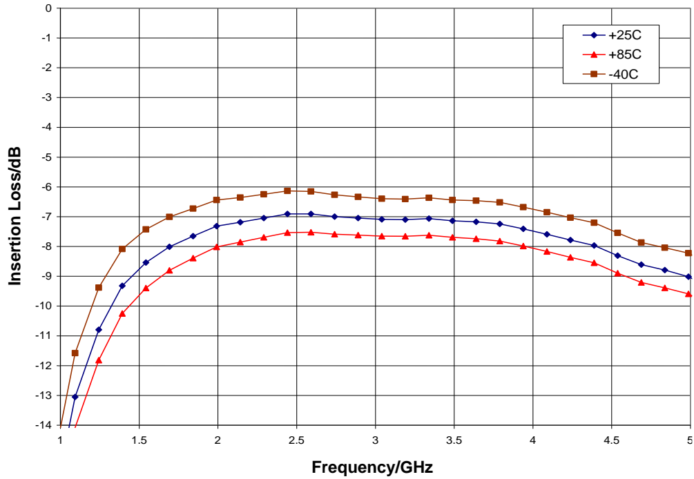
Insertion Loss vs. Temperature, Reference State, V_{ee} = -3.0\text{ V}
