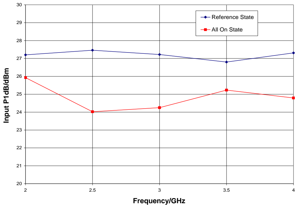
Input P1dB, V_{ee} = -3.0\text{ V}
