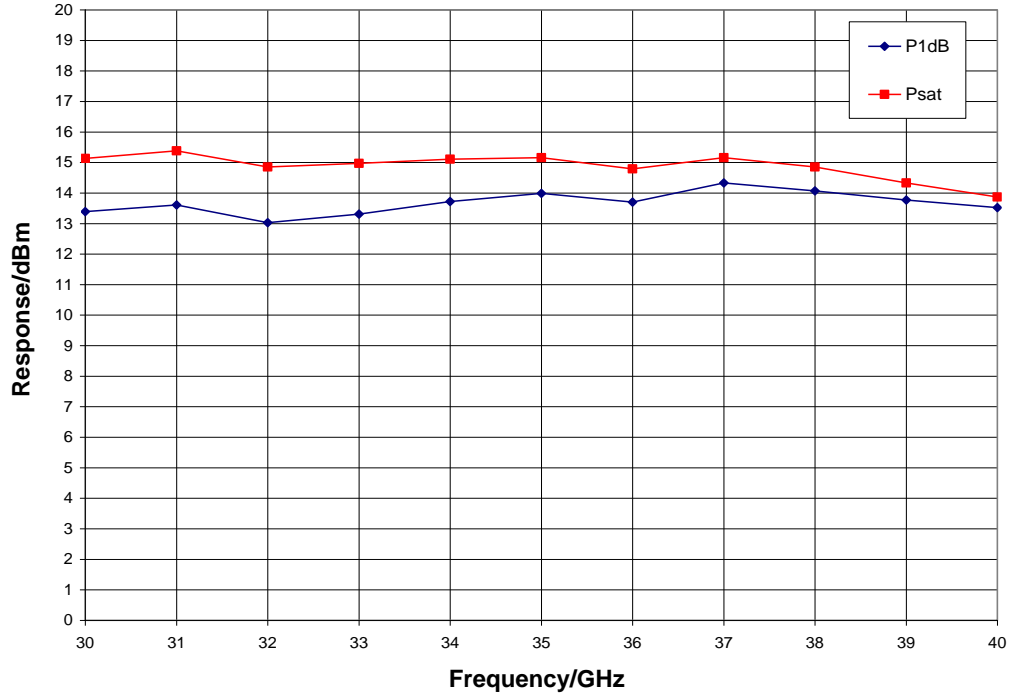
Output Power, V_{dd} = 3.0\text{ V} , V_{gg} = 3.0\text{ V} , T_A = 25\text{ °C}
