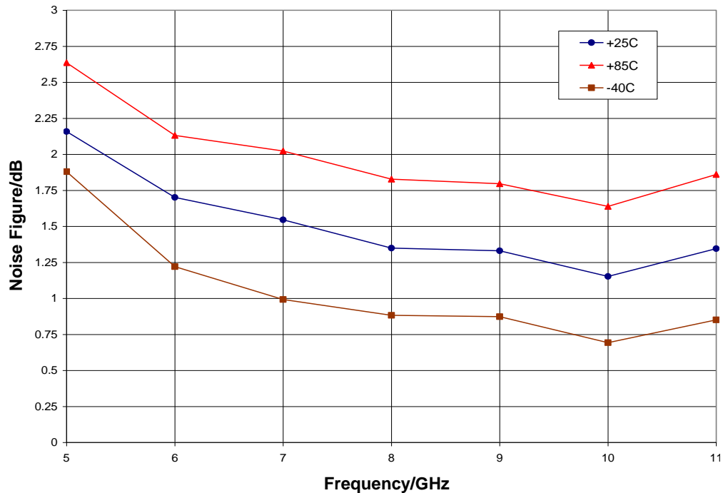
Noise Figure vs. Temperature, V_{dd} = 3.6\text{ V}
