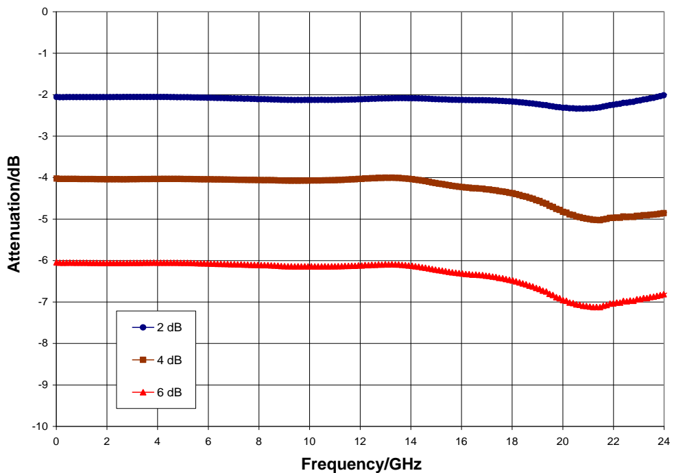
Normalized Attenuation (all states), T_A = 25^\circ C
