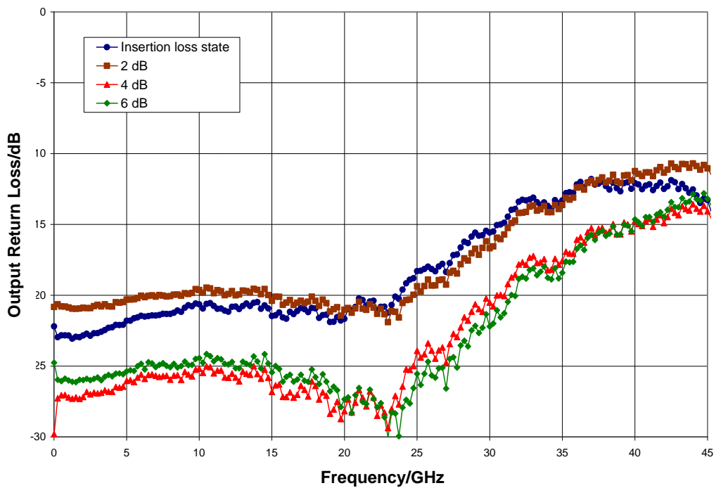
Output Return Loss (all states), T_A = 25^\circ\text{C}
