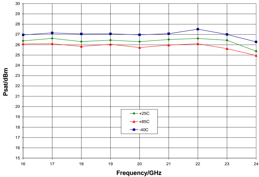
Psat vs. Temperature, V_{dd} = 5\text{ V}
