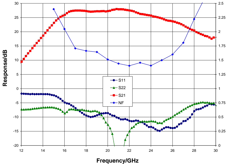
Narrow-band Performance, V_{dd} = 3.0\text{ V} , V_{gg} = 1.5\text{ V} , I_{dd} = 27\text{ mA} , T_A = 25^\circ\text{ C}
