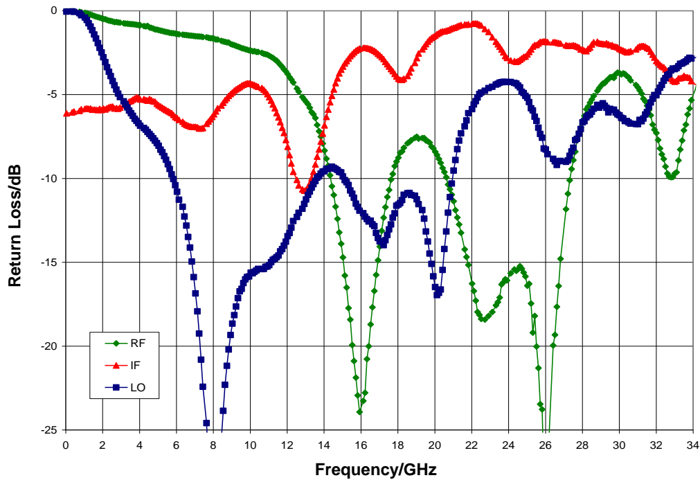
Return Loss, LO = -2 dBm, T A = 25° C
