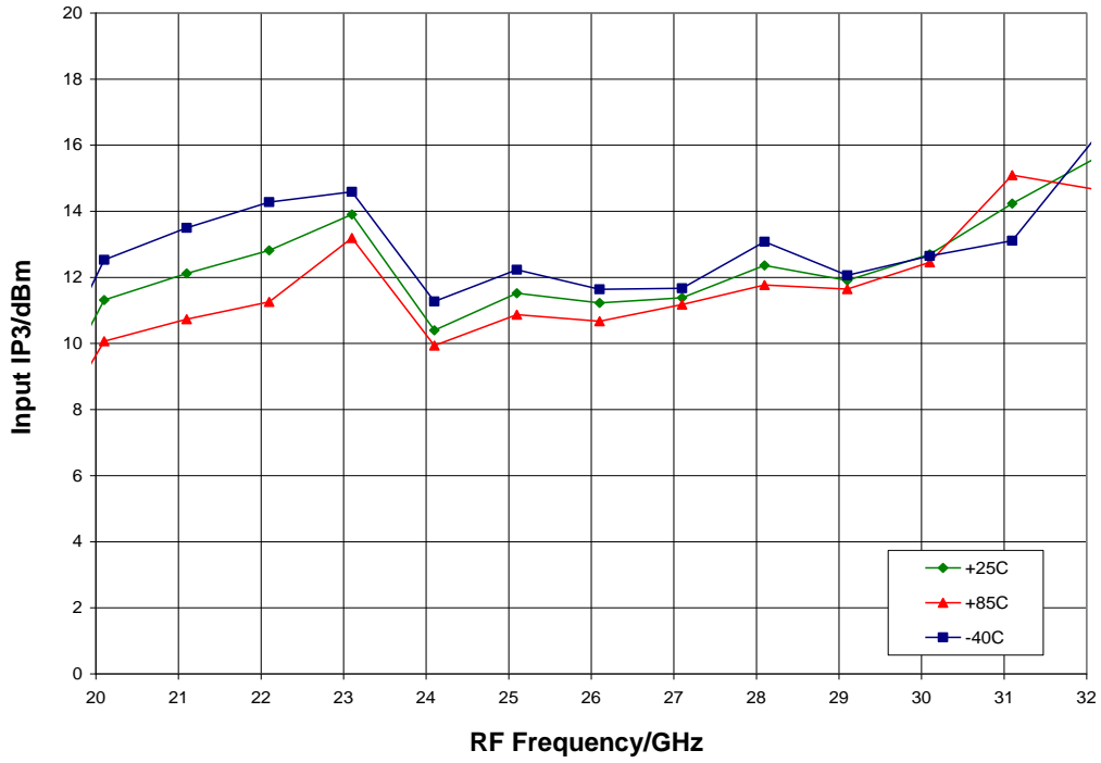
Input IP3 vs. Temperature, LO = -2 dBm
