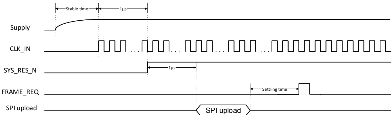
FIGURE 8: START-UP SEQUENCE FOR 12-BIT MODE
