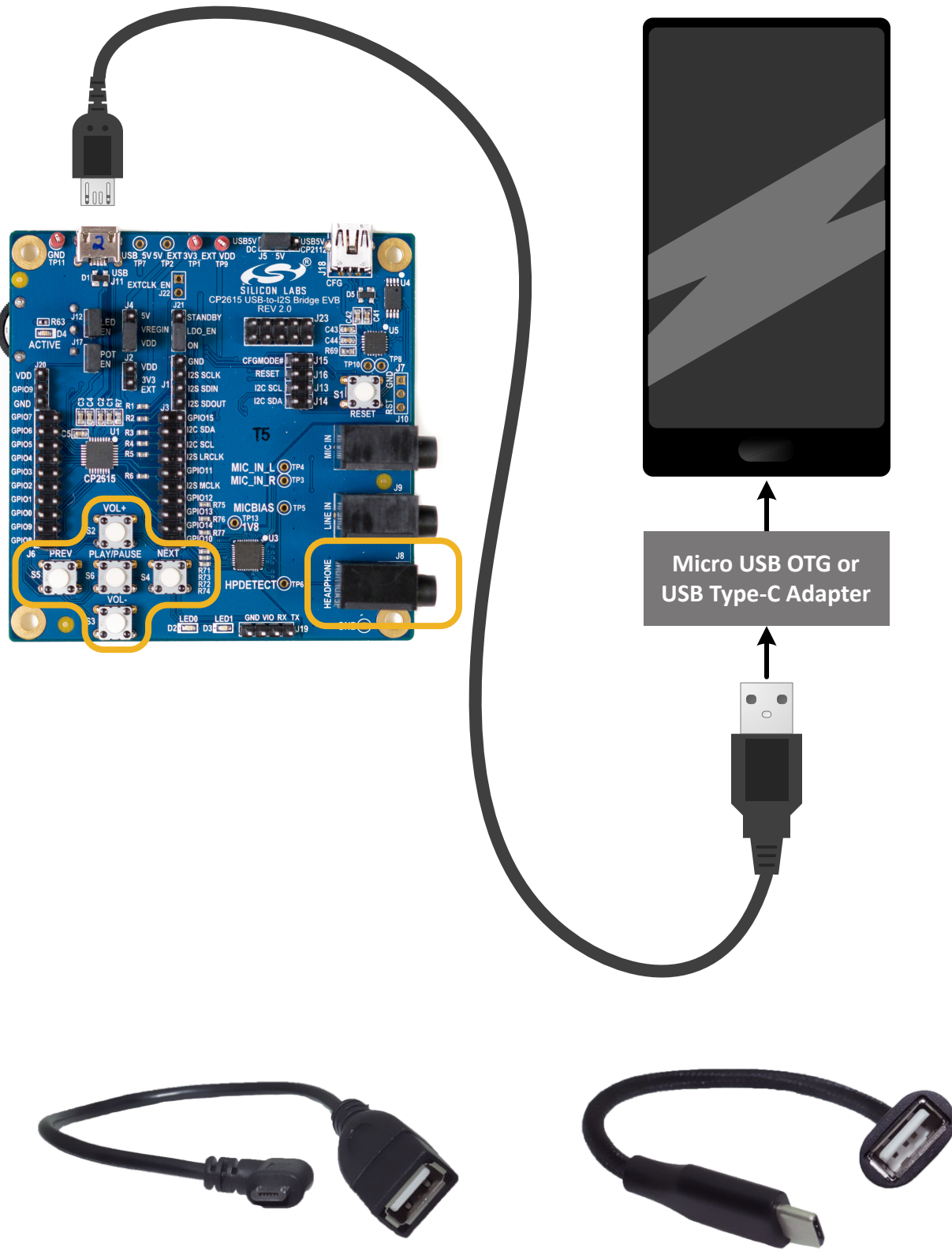
Micro OTG Adapter Cable
