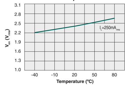
Typical Output Voltage Drop vs. Temperature
