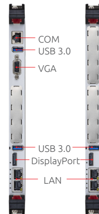
cPCI-6540
