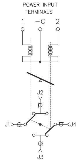
SCHMATIC
