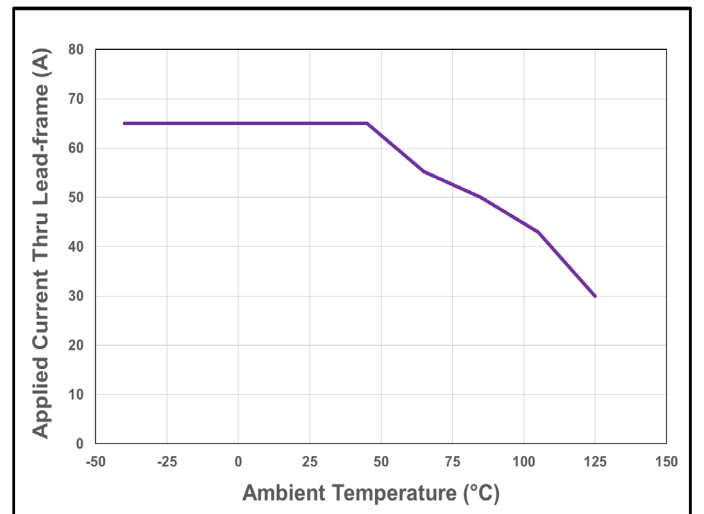
Figure 44. CT431 Current De-rating Curve for 65 A bc
