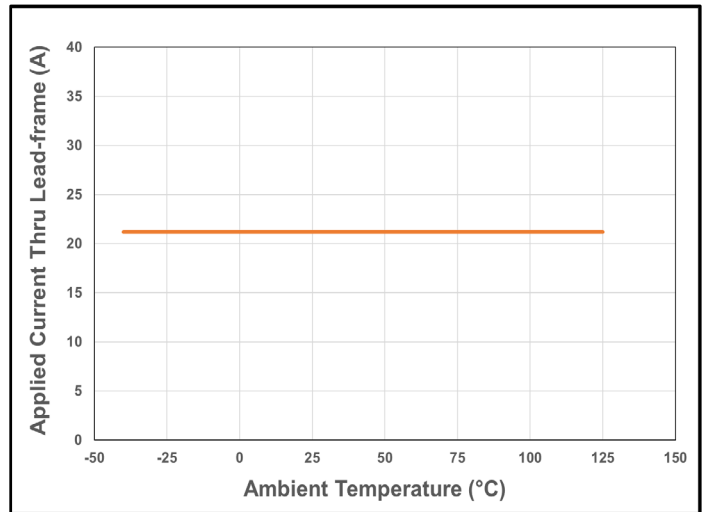
Figure 32. CT431 Current De-rating Curve for 30 A PK (21.2 A DC )
