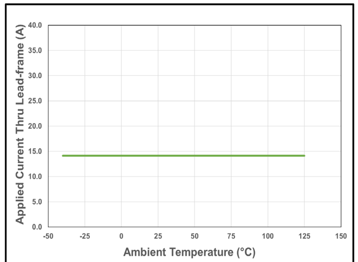
Figure 24. CT431 Current De-rating Curve for 20 A_{PK} (14.1 A_{DC} )
