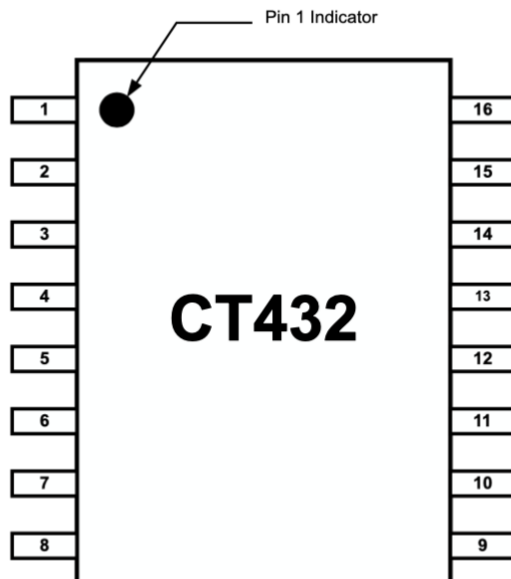
Figure 2. CT432 Pin-out Diagram for 16-lead SOIC-Wide Package (Top-Down View)
