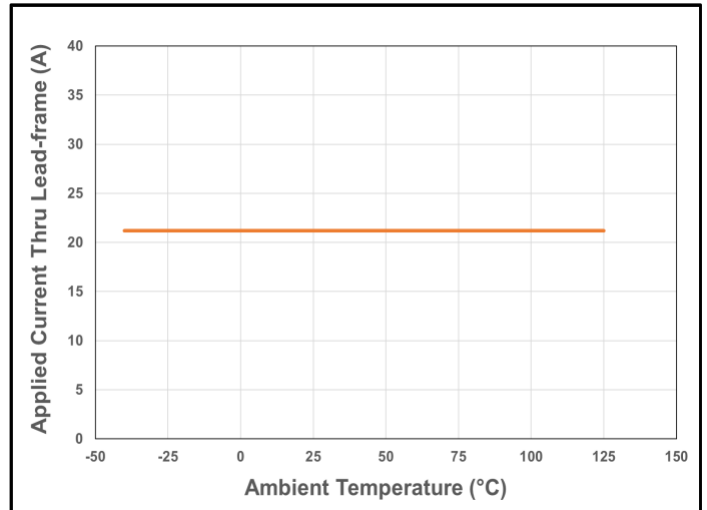
Figure 19. CT432 Current De-rating Curve for 30 A PK (21.2 A RMS )
