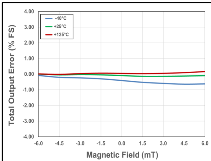
Figure 13. Total Output Error vs. B Field vs. Temperature
