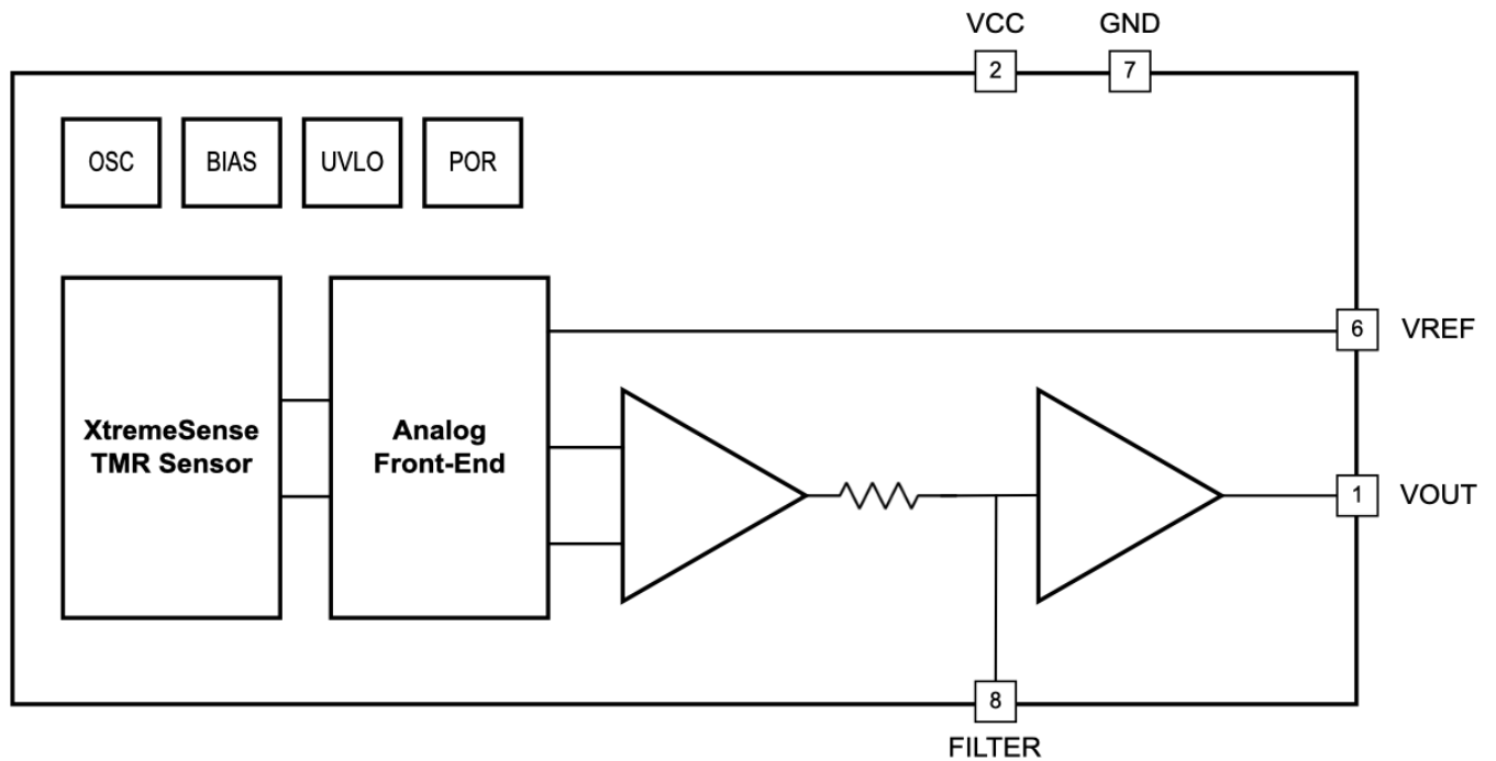
Figure 2. CT452 Functional Block Diagram for TSSOP-8
