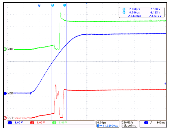
Figure 10. CT452 Startup Waveforms for V_{OQ} = 2.50\text{ V} (Bipolar Sensor Version)
