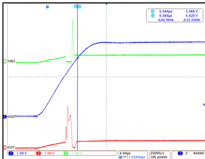
Figure 9. CT452 Startup Waveforms for V_{OQ} = 0.50\text{ V} (Unipolar Sensor Version)
