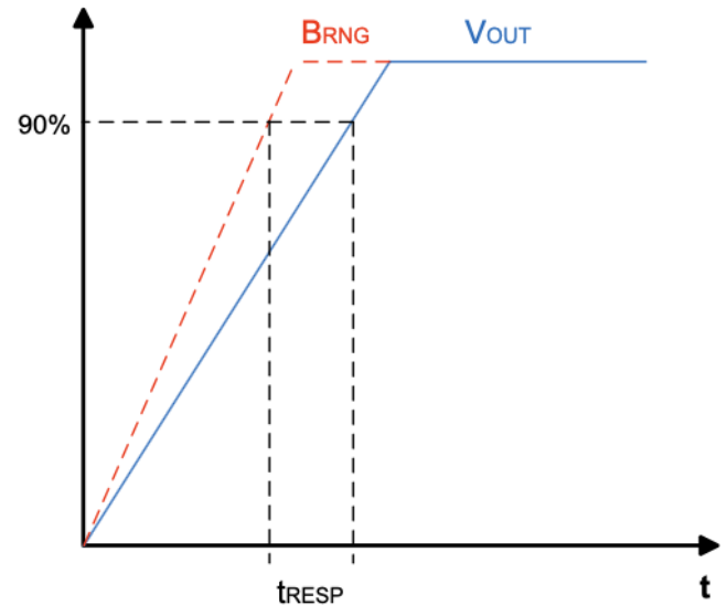
Figure 22. CT452 Response Time Curve
