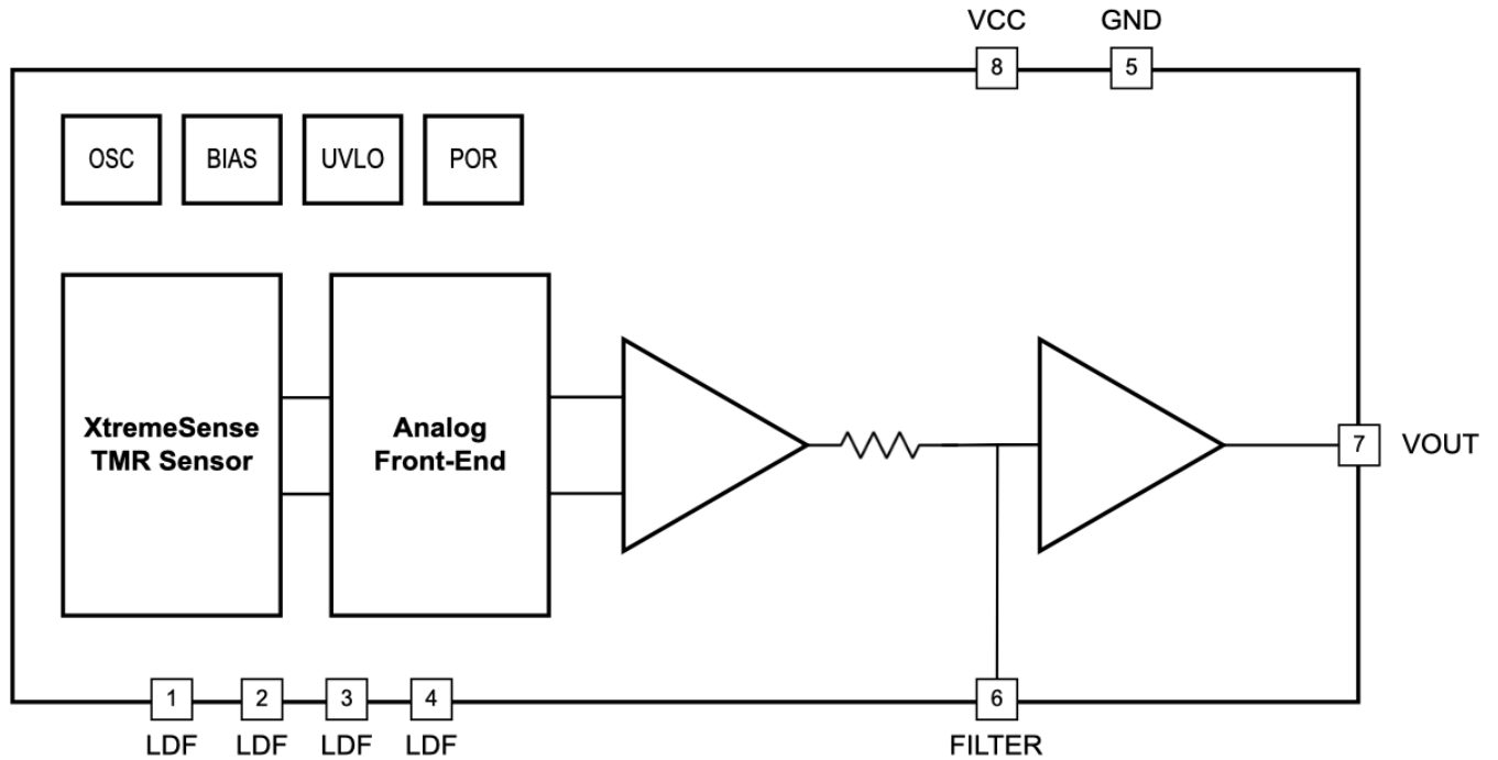
Figure 1. CT452 Functional Block Diagram for SOIC-8
