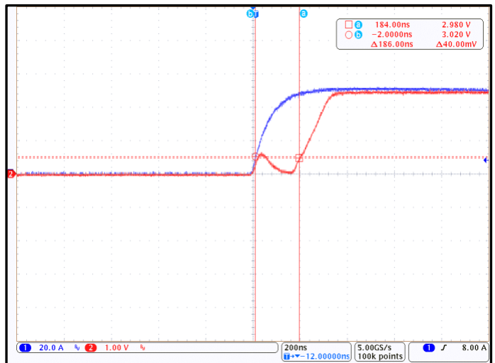
Figure 7. CT432 Propagation Delay; I_P = 50\text{ A}_{PK} and C_L = 100\text{ pF} (Blue = I_{LCC} , Red = V_{OUT} )
