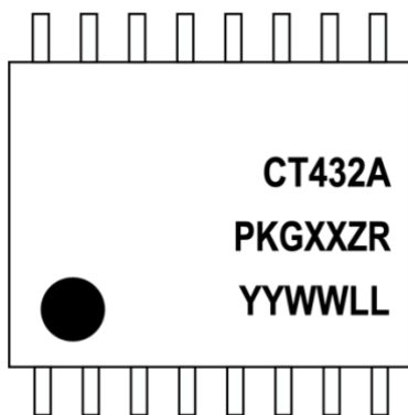
Figure 42. CT432 Device Marking for 16-lead Package
