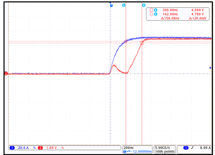
Figure 5. CT432 Response Time; I_P = 50\text{ A}_{PK} and C_L = 100\text{ pF} (Blue = I_{LCC} , Red = V_{OUT} )
