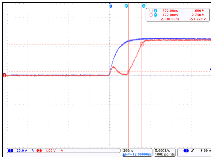
Figure 6. CT432 Rise Time; I_P = 50\text{ A}_{PK} and C_L = 100\text{ pF} (Blue = I_{LCC} , Red = V_{OUT} )
