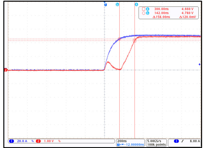
Figure 5. CT432 Response Time; I_P = 50\text{ A}_{PK} and C_L = 100\text{ pF} (Blue = I_{CC} , Red = V_{OUT} )
