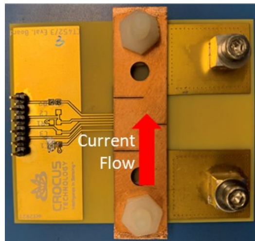
FIGURE 5. CTD453 WITH BUSBAR
