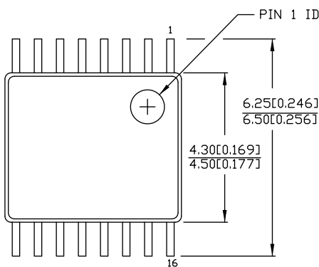
Figure 13. 16-pin TSSOP (4.40 mm Body) Z16.173/ZZ16.173 Package Outline, 51-85091
