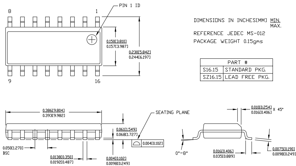
Figure 10. 16-Pin (150-Mil) SOIC S16 and SZ16
