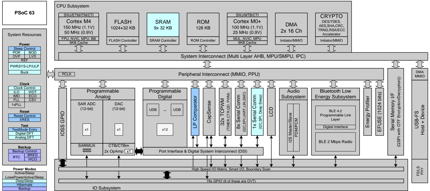
Figure 2. 框图
