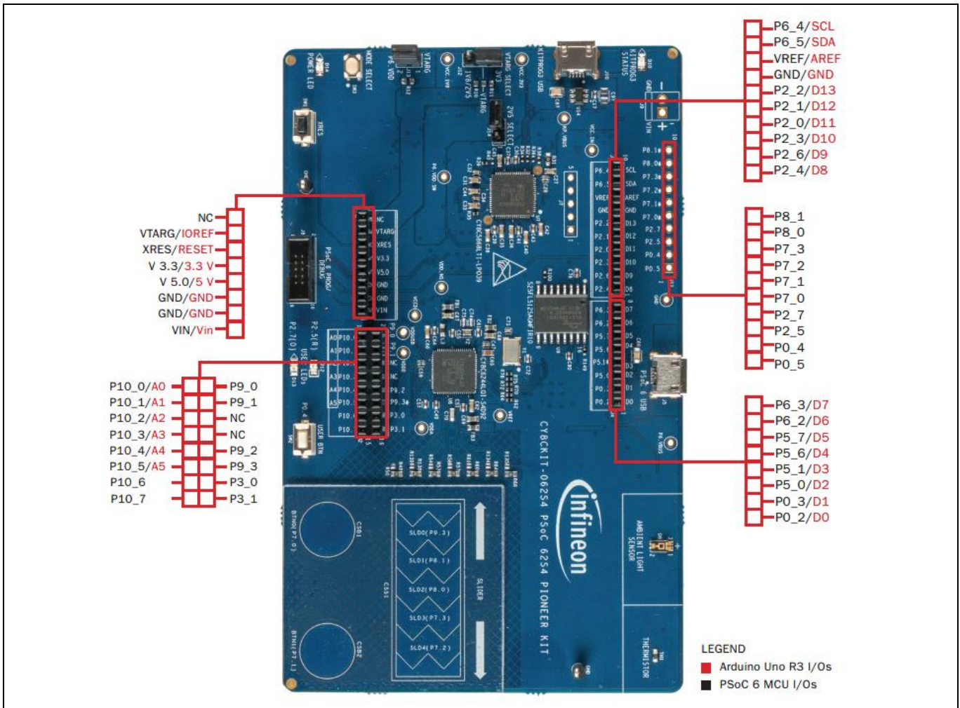
Figure 2 CY8CKIT-062S4 PSoC™ 62S4 pioneer board pinout
