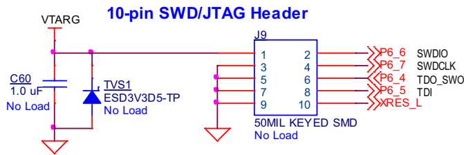
Figure 5-13. 10-pin SWD/JTAG Header
