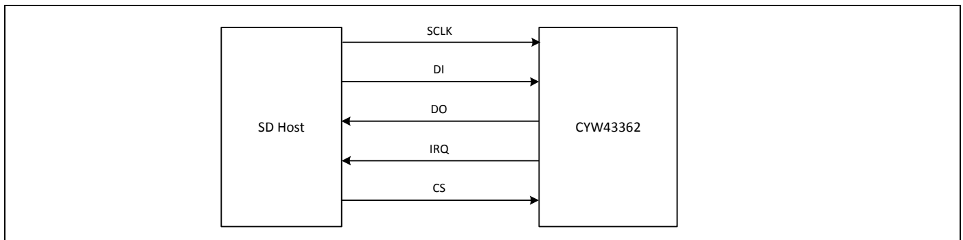
Figure 8. Signal Connections to SDIO Host (gSPI Mode)
