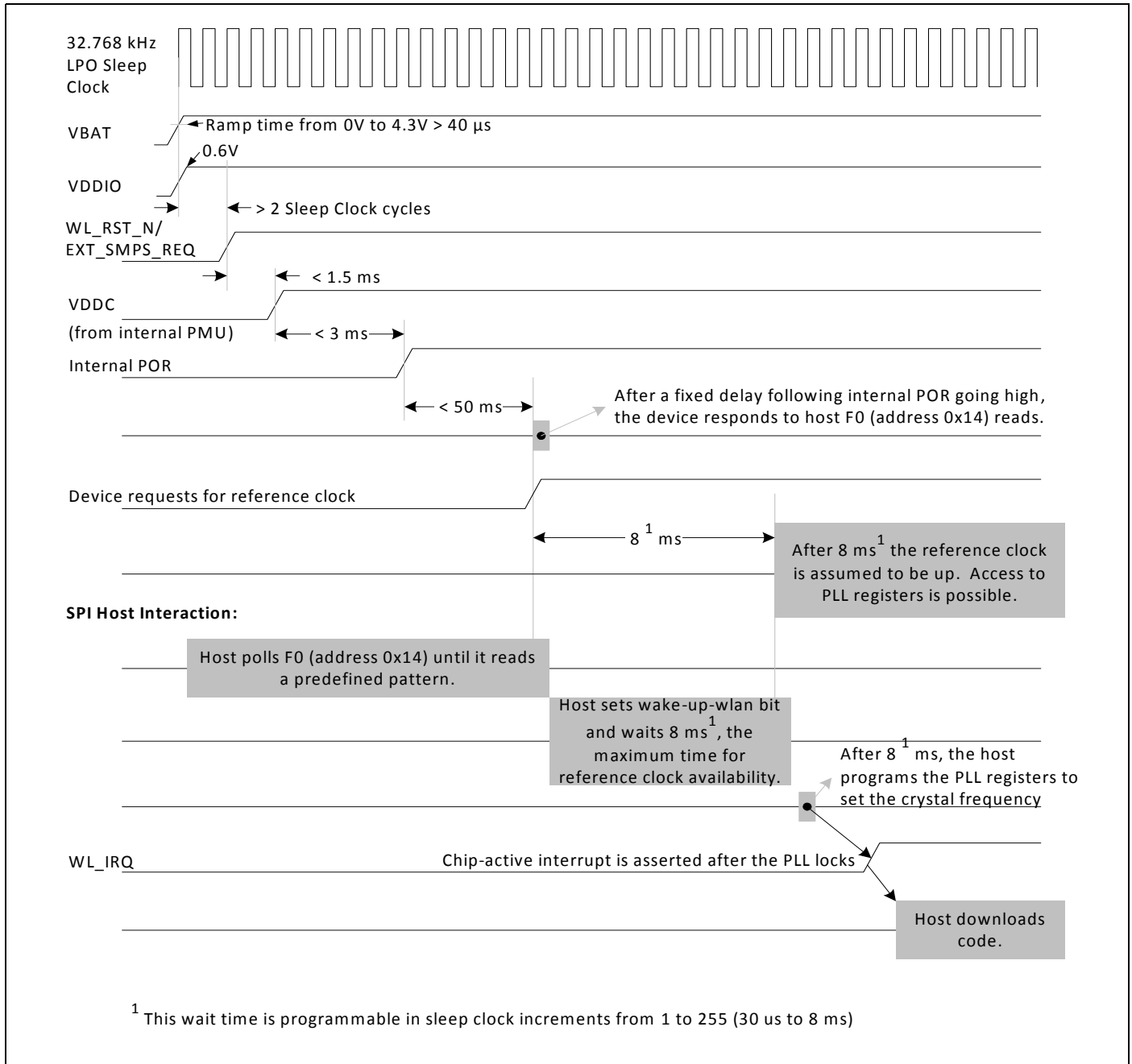
Figure 14. WLAN Boot-Up Sequence
