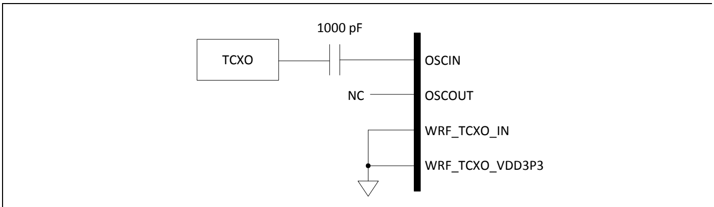
Figure 5. Recommended Circuit to Use with an External Shared TCXO
