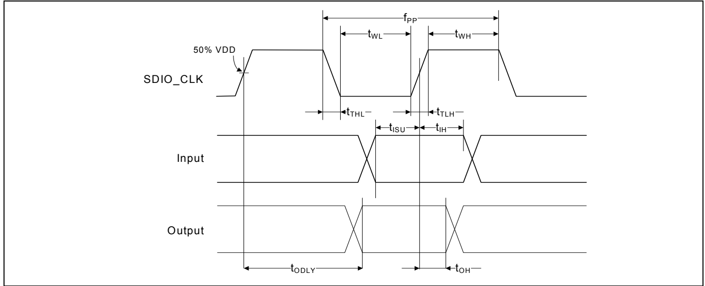
Figure 25. SDIO Bus Timing (High-Speed Mode)
