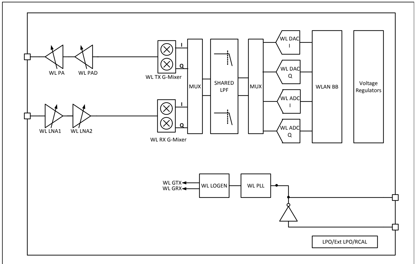
Figure 19. Radio Functional Block Diagram
