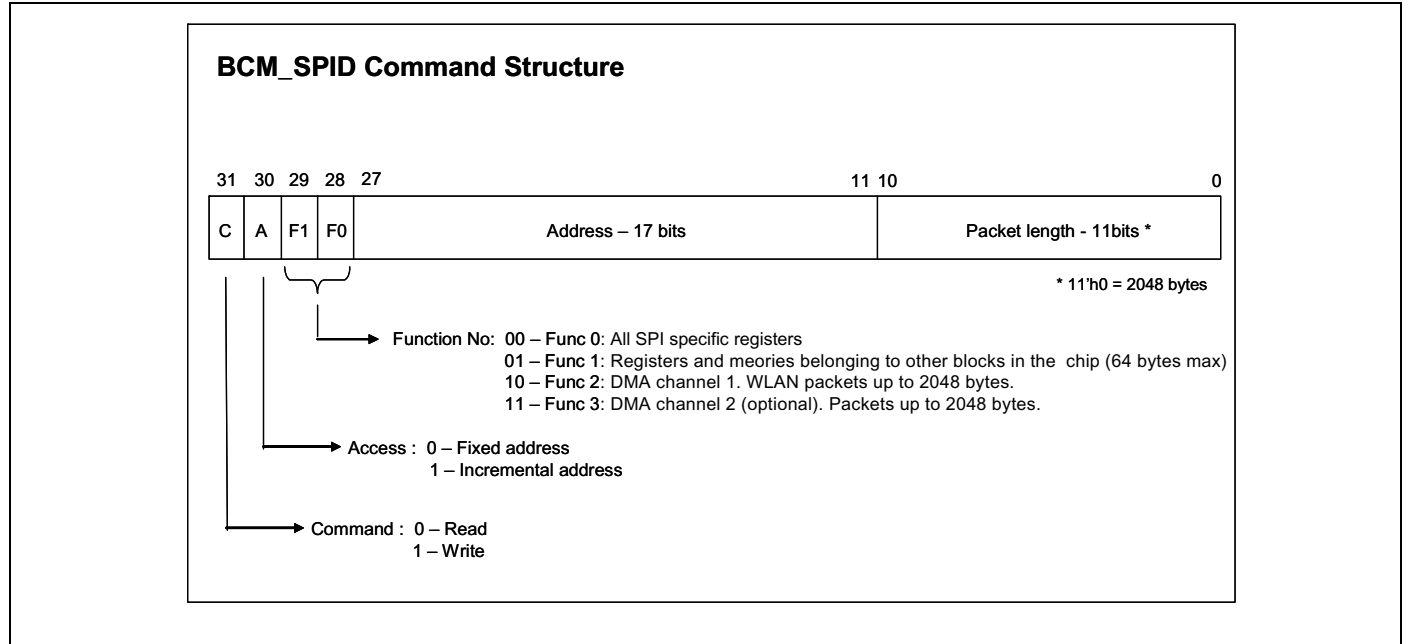
Figure 11. gSPI Command Structure
