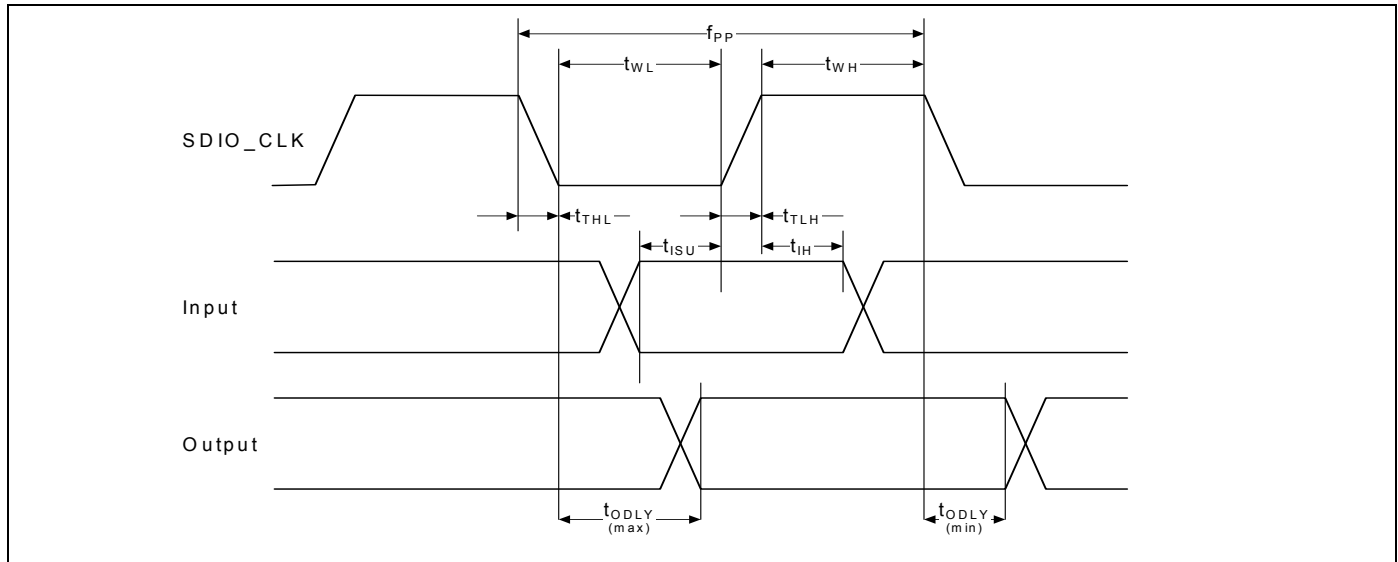
Figure 24. SDIO Bus Timing (Default Mode)
