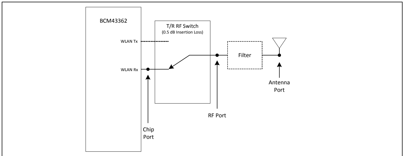
Figure 22. RF Port Location
