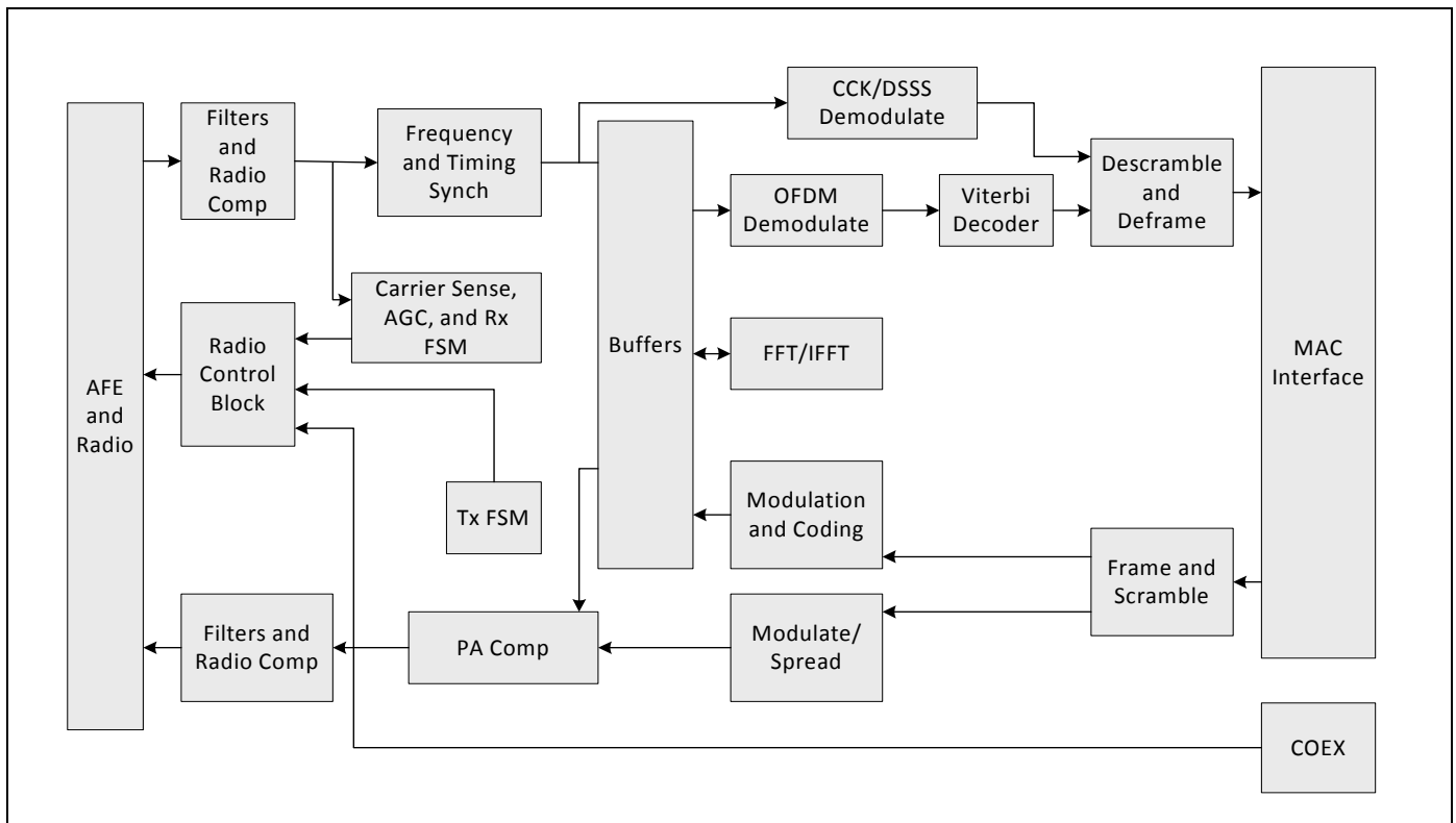
Figure 17. WLAN PHY Block Diagram
