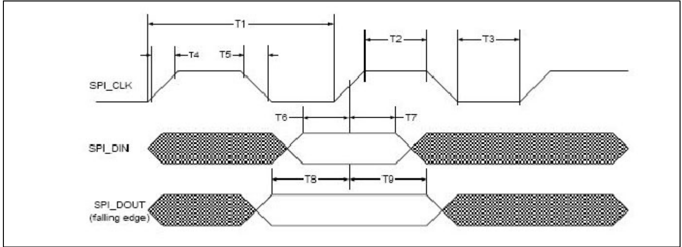
Figure 26. gSPI Timing
