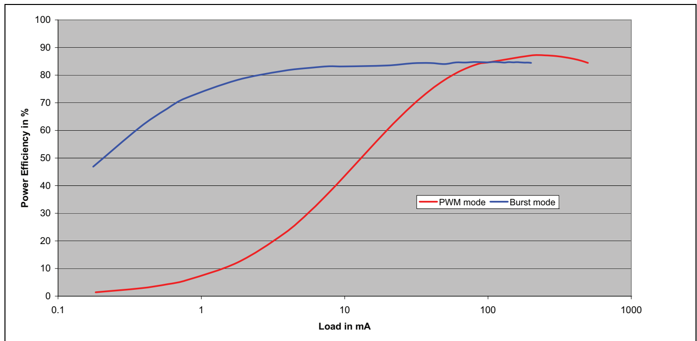
Figure 23. CBUCK Efficiency
