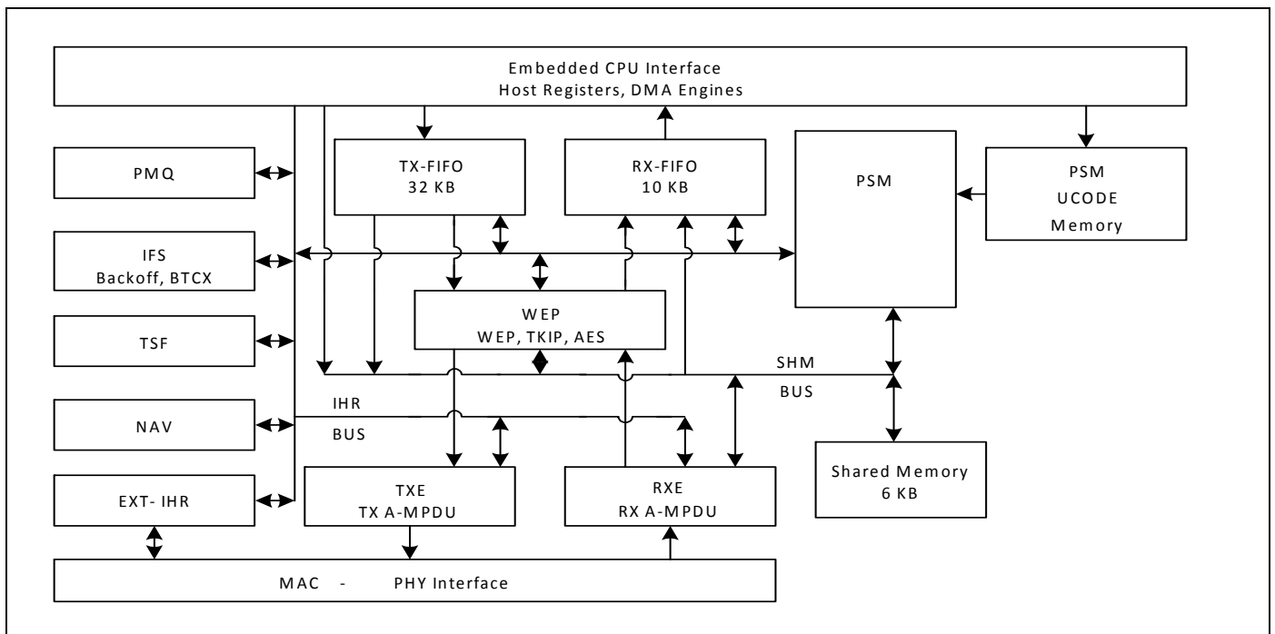
Figure 16. WLAN MAC Architecture
