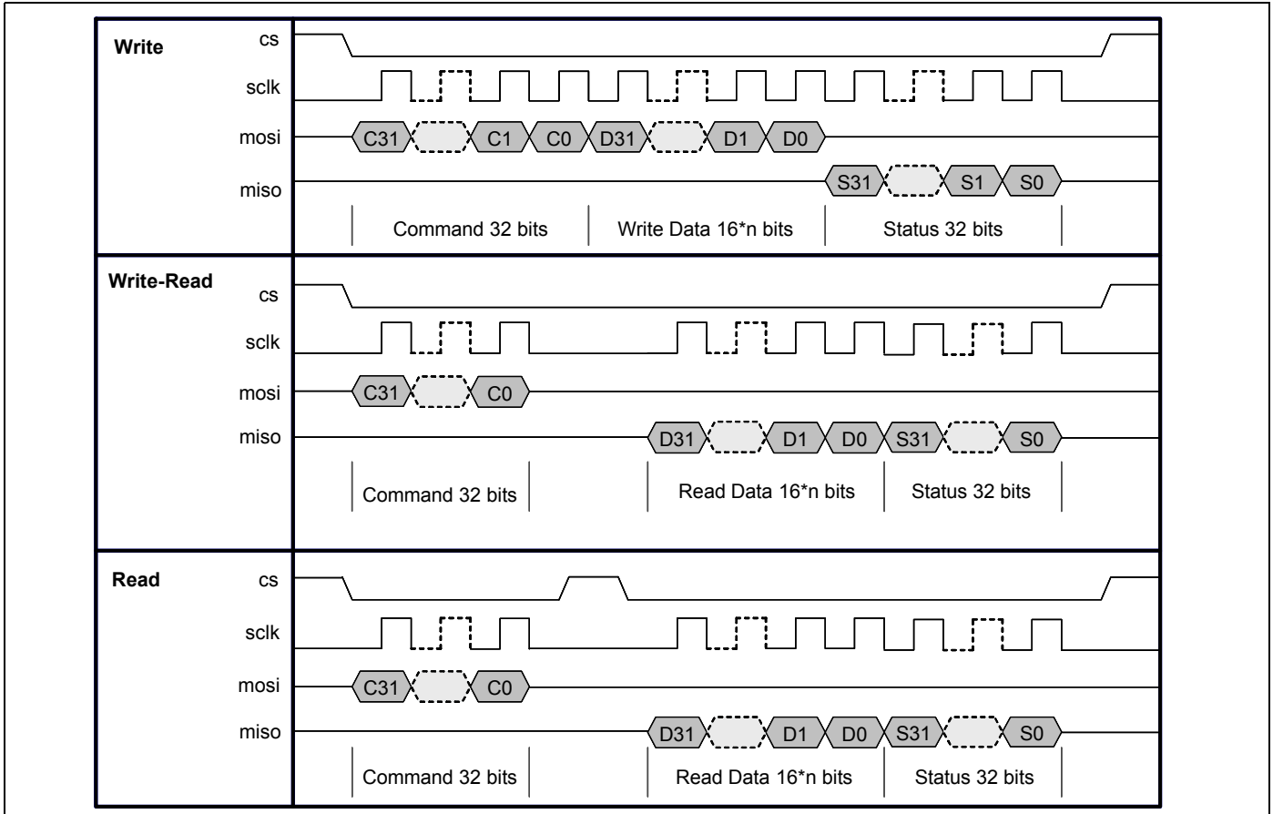
Figure 13. gSPI Signal Timing with Status (Response Delay = 0)
