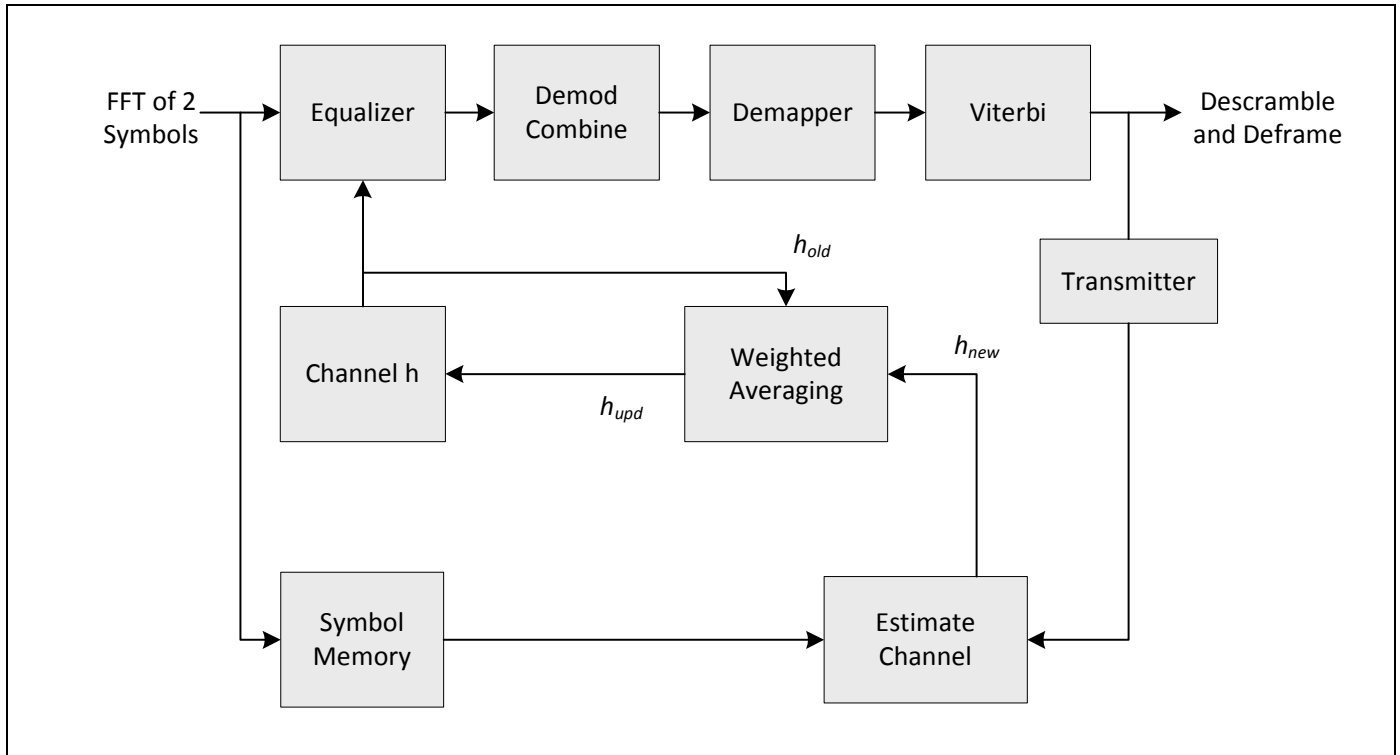
Figure 18. STBC Receive Block Diagram
