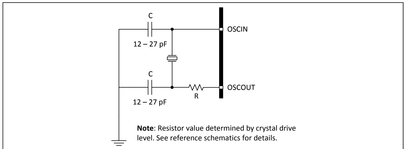
Figure 3. Recommended Oscillator Configuration
