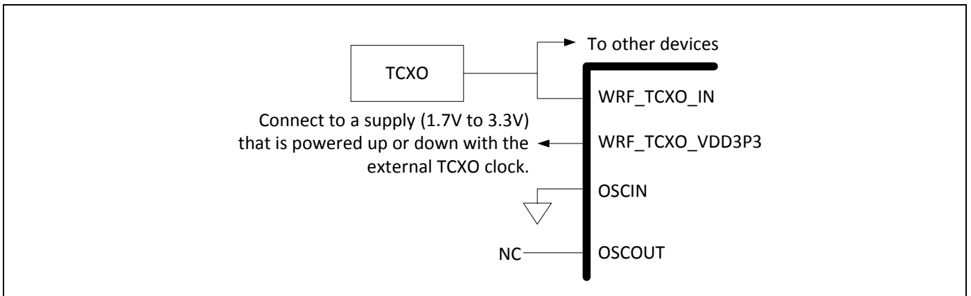
Figure 5. Recommended Circuit to Use with an External Shared TCXO
