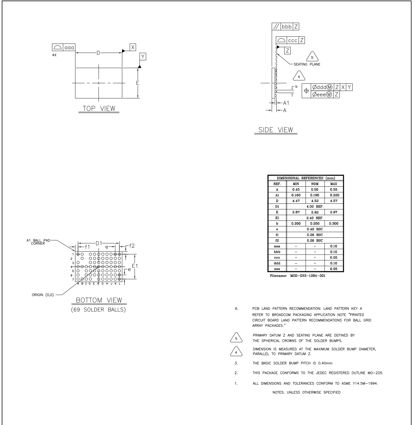
Figure 27. 69-Ball WLBGA Mechanical Information
