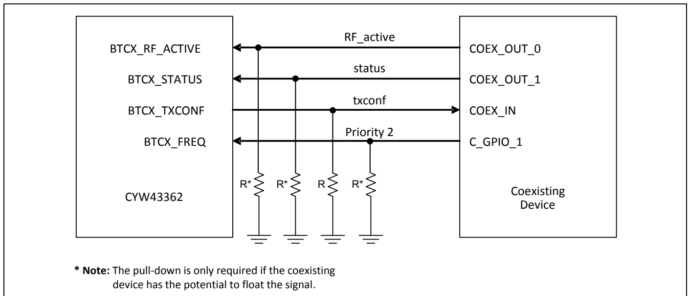
Figure 15. 4-Wire Coexistence Wiring
