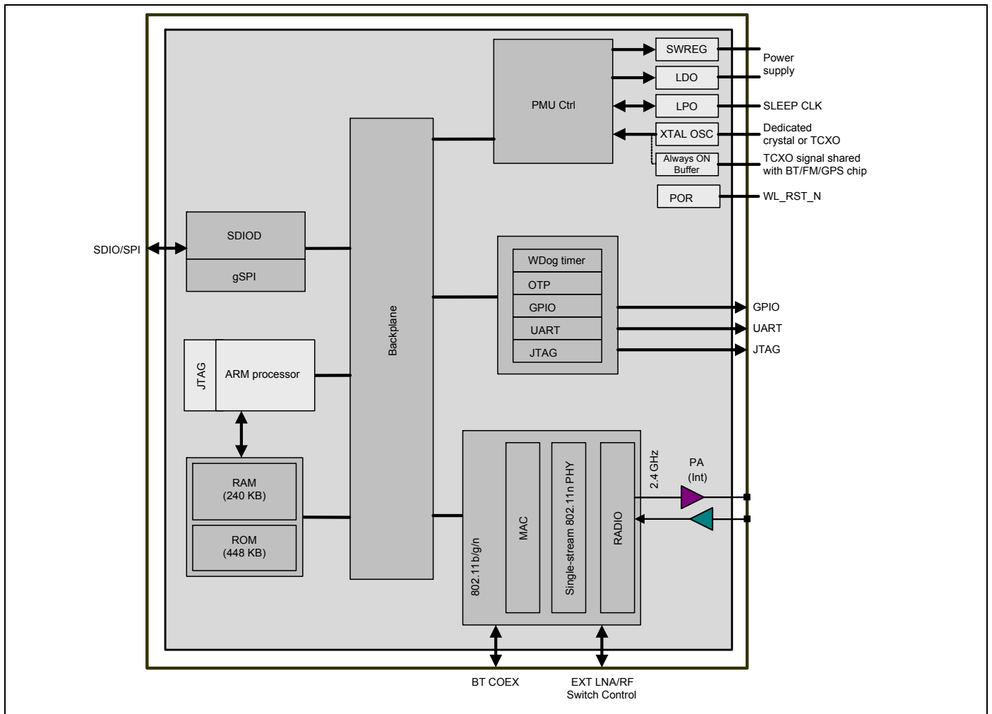
Figure 1. CYW43362 Block Diagram
