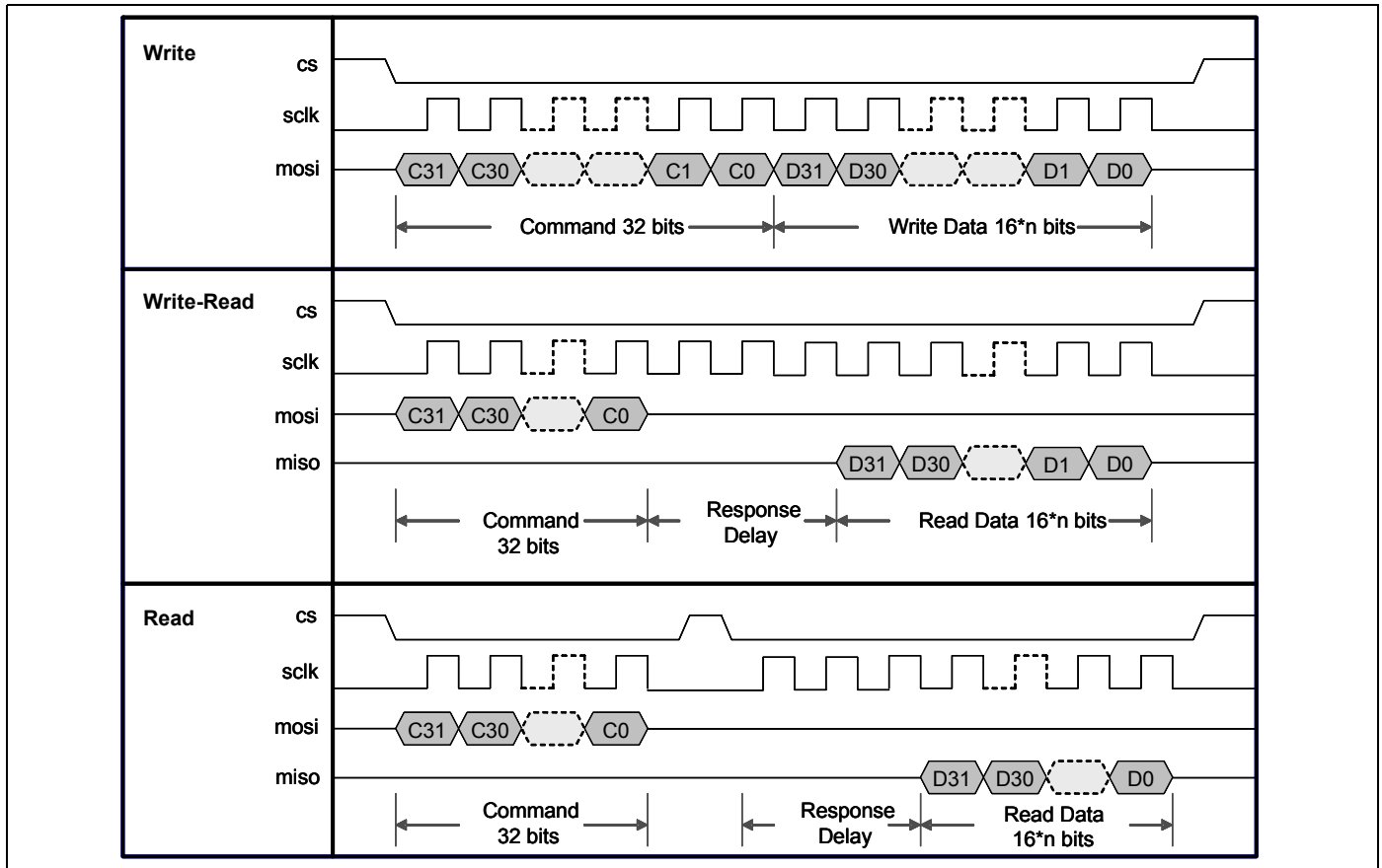
Figure 12. gSPI Signal Timing Without Status
