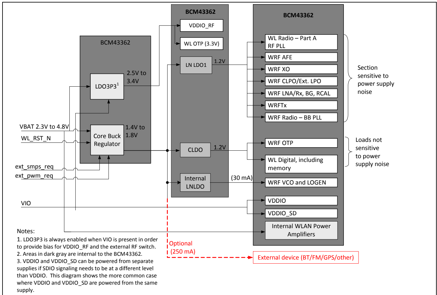
Figure 2. Power Topology
