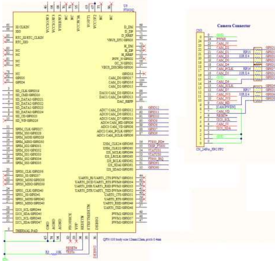
Figure 6 - Camera Interface
