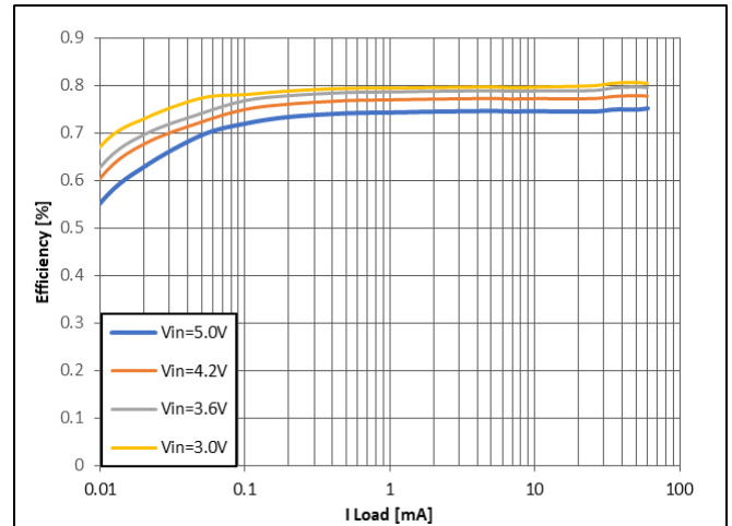
Figure 11: Buck V OUT = 0.7 V
