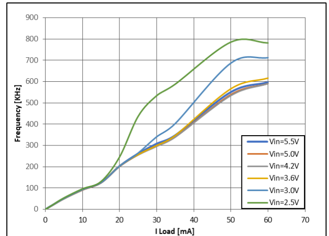
Figure 15: Buck V OUT = 0.7 V
