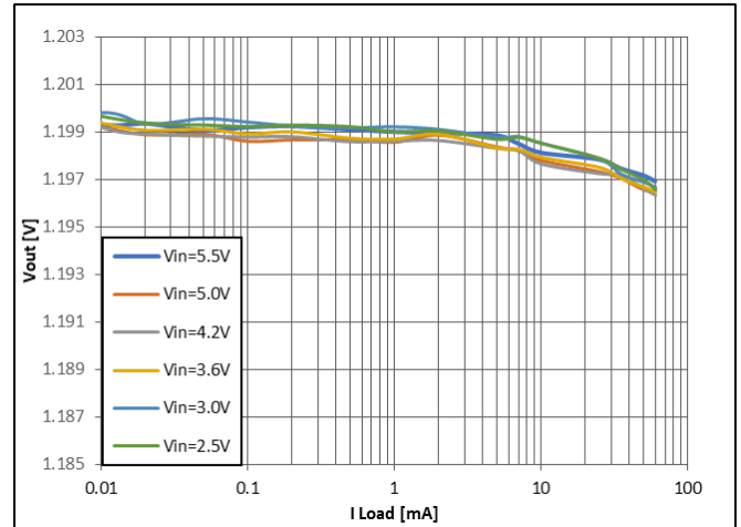
Figure 191: Buck V OUT = 1.2 V
