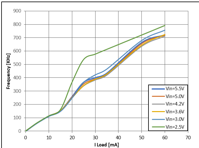
Figure 144: Buck V OUT = 0.9 V
