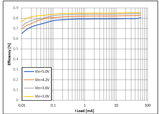
Figure 9: Buck V OUT = 1.2 V
