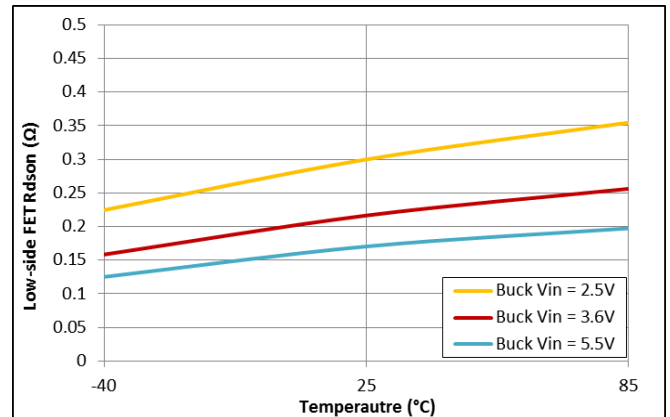
Figure 7: Low-Side FET
