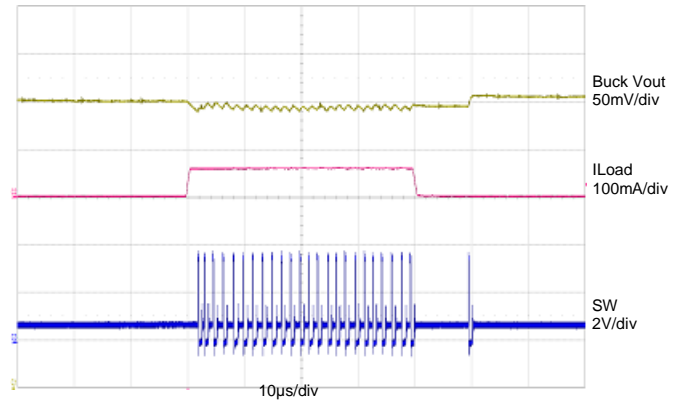
Figure 29: Buck I_{LOAD} = 0.5 \text{ mA} to 60 \text{ mA} to 0.5 \text{ mA} ( 0.1 \text{ A}/\mu\text{s} ); Buck V_{IN} = 3.6 \text{ V} , Buck V_{OUT} = 0.7 \text{ V}
