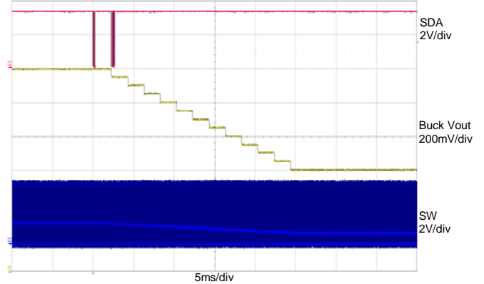
Figure 261: Buck V_{OUT} 1.2 V to 0.6 V; Buck V_{IN} = 3.6 V, Buck I_{LOAD} = 60 mA
