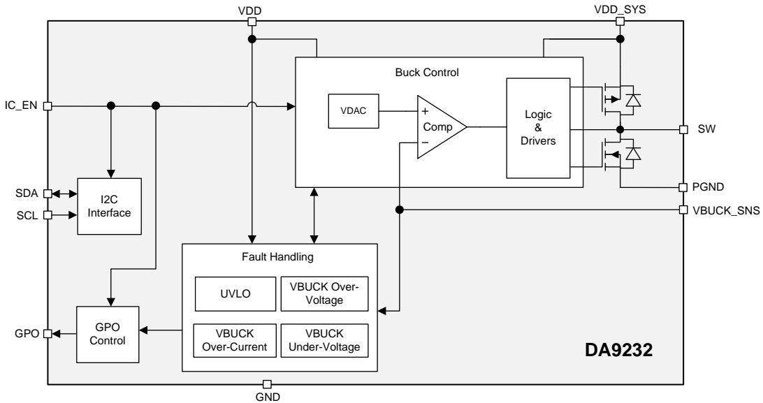
Figure 1: Block Diagram
