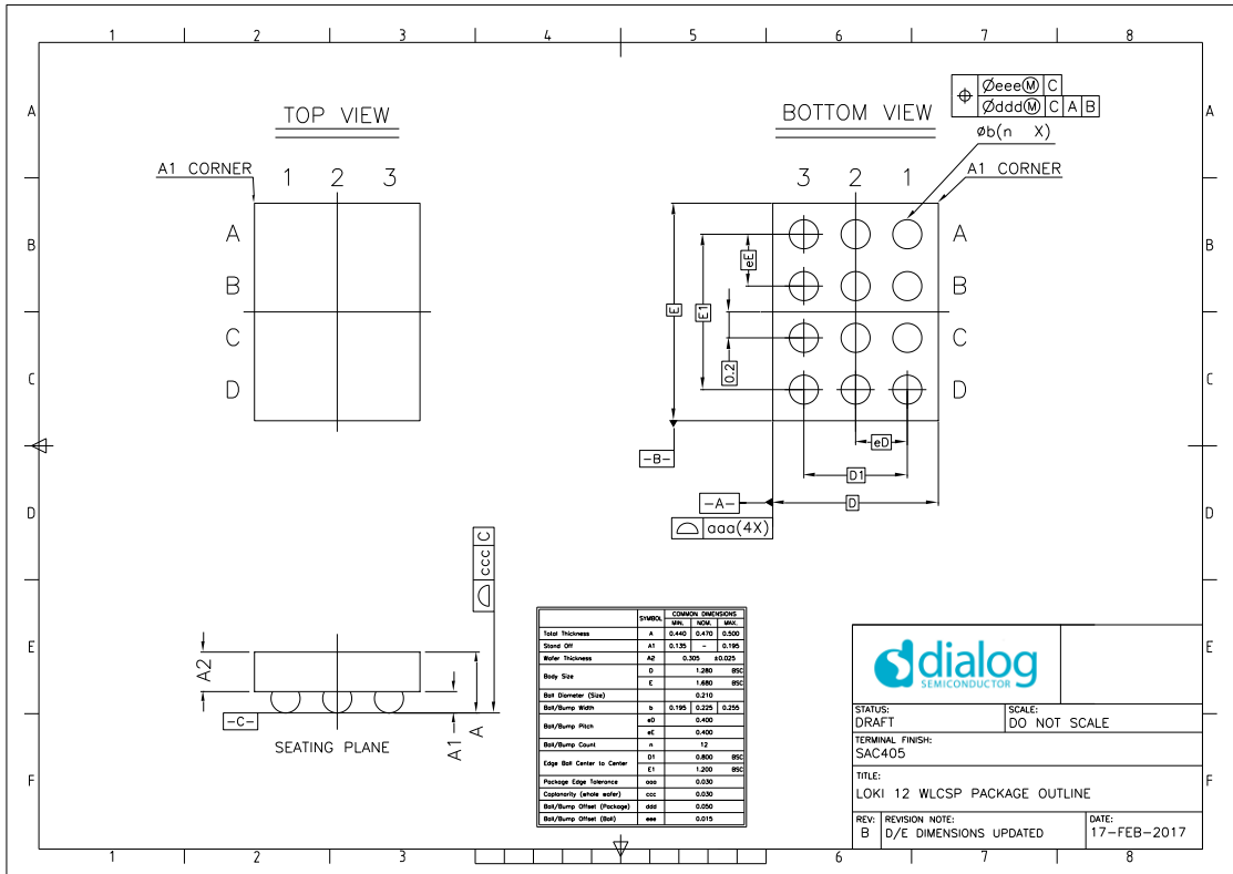
Figure 38: Package Outline Drawing
