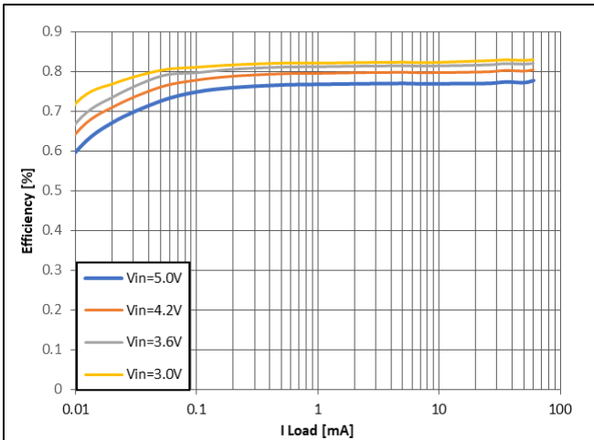
Figure 10: Buck V OUT = 0.9V
