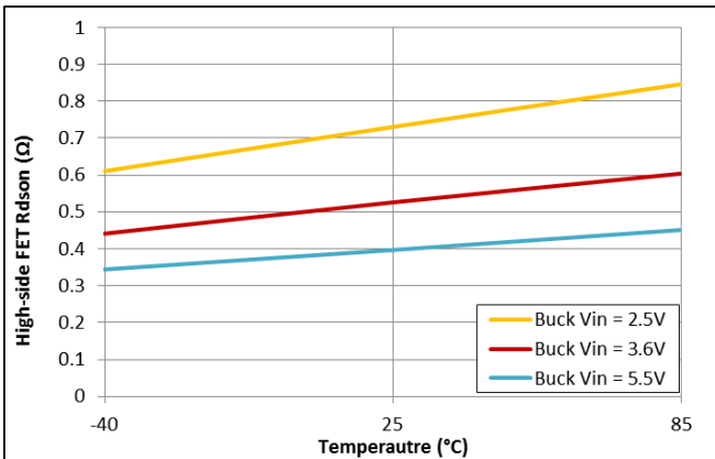
Figure 6: High-Side FET
