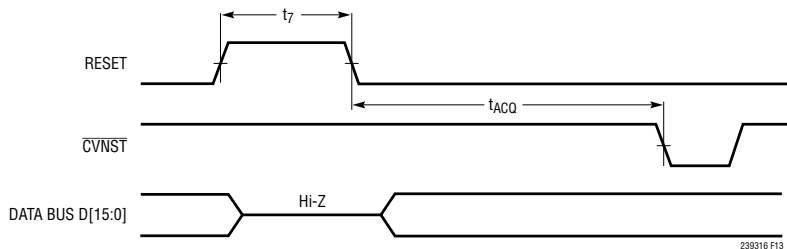
Figure 13. RESET Pin Timing
