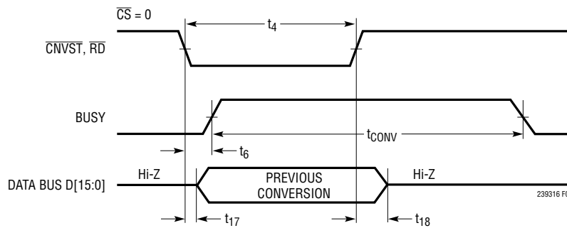
Figure 10. Read the Parallel Data During the Conversion
