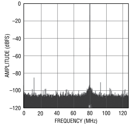
LTC2152-14: 32K Point FFT, f_{IN} = 171\text{MHz} , -1\text{dBFS} , 250Mps
