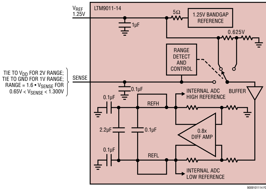
Figure 8. Reference Circuit
