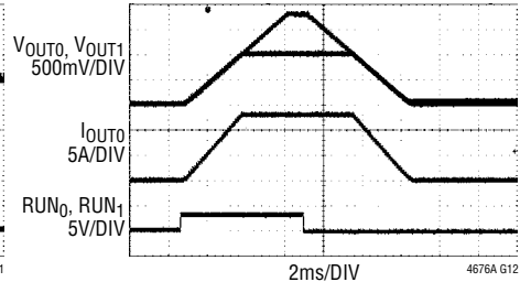
FIGURE 69 CIRCUIT AT 12\text{V}_{\text{IN}} . 77\text{m}\Omega LOAD ON \text{VOUT}_0 . NO LOAD ON \text{VOUT}_1 . \text{TON\_RISE}_0 = 3\text{ms} , \text{TON\_RISE}_1 = 5.297\text{ms} , \text{TOFF\_DELAY}_1 = 0\text{ms} , \text{TOFF\_DELAY}_0 = 2.43\text{ms} , \text{TOFF\_FALL}_1 = 5.328\text{ms} , \text{TOFF\_FALL}_0 = 3\text{ms} , \text{ON\_OFF\_CONFIG}_n = 0\text{x}1\text{E}
