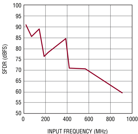
SFDR vs Input Frequency, -1dBFS, 1.5V Range, 250Msps
