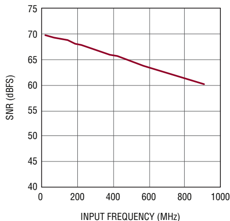
SNR vs Input Frequency, -1dBFS, 1.5V Range, 250Msps
