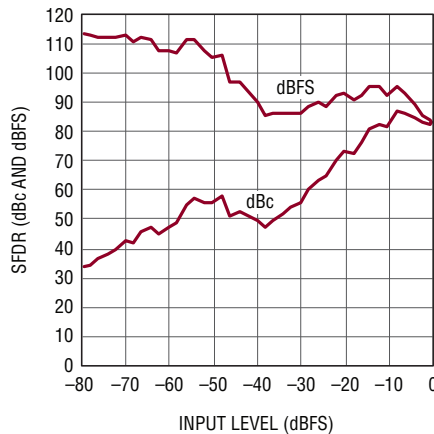
SFDR vs Input Level, f_{IN} = 70\text{MHz} , 1.5V Range, 250Msps
