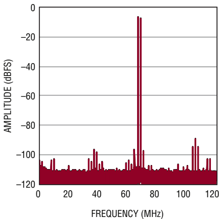
64k Point 2-Tone FFT, f_{IN} = 71.1\text{MHz} and 69MHz, -7dBFS, 250Msps
