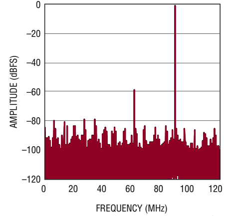
64k Point FFT, f_{IN} = 907.1\text{MHz} , -1dBFS, 250Msps
