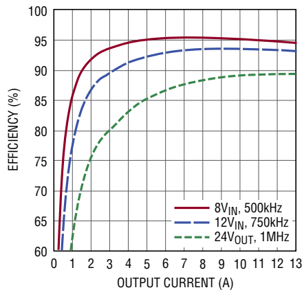
Efficiency vs Output Current, V_{OUT1} = 5V , V_{OUT0} = \text{OFF} , V_{IN} = SV_{IN} = V_{INn} , INTV_{CC} Open
